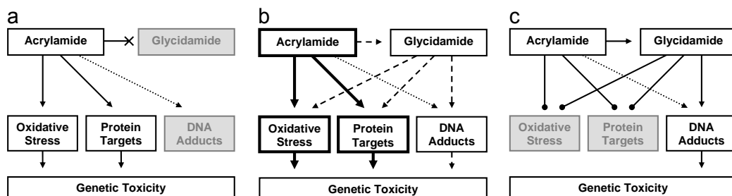
Figure 3: A series of diagrams demonstrating the possible effects of (a) lack of metabolic activation, (b) high exposure level in vivo and (c) low exposure level in vivo . The cross in (a) represents lack of metabolism, the spots in (c) represent failure to reach the hypothesised threshold, and the thick / dashed lines in (b) represent relative contributions of the various mechanisms of action.
