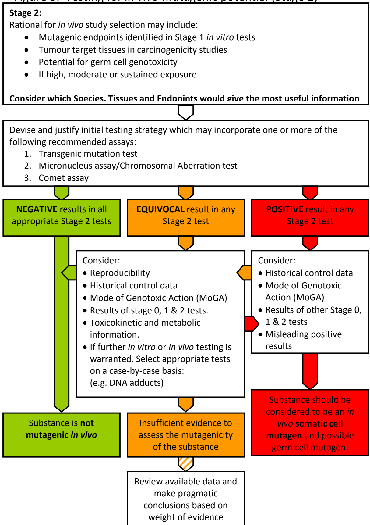
Figure 3: Testing for in vivo mutagenic potential (Stage 2)
